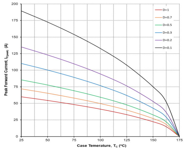
Figure 8. Current Derating
