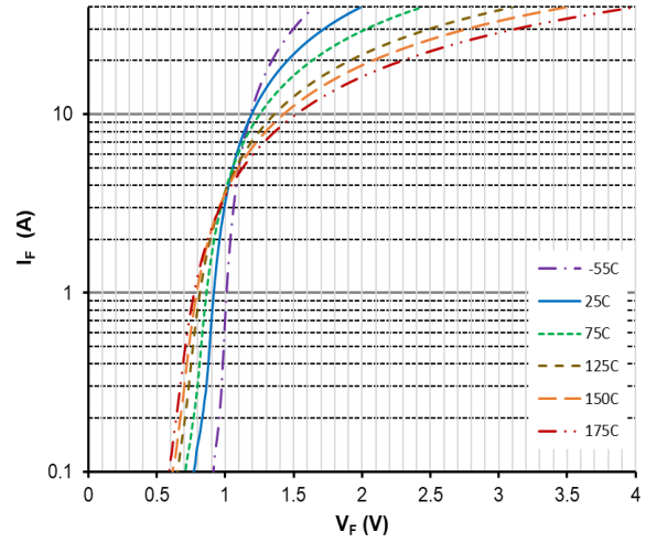
Figure 2. Forward Characteristics
