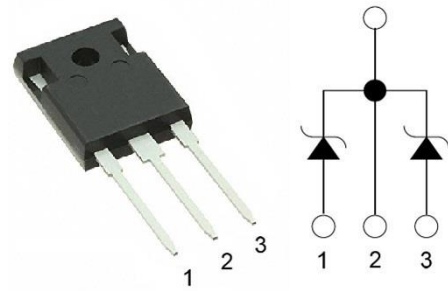
TO-247-3
