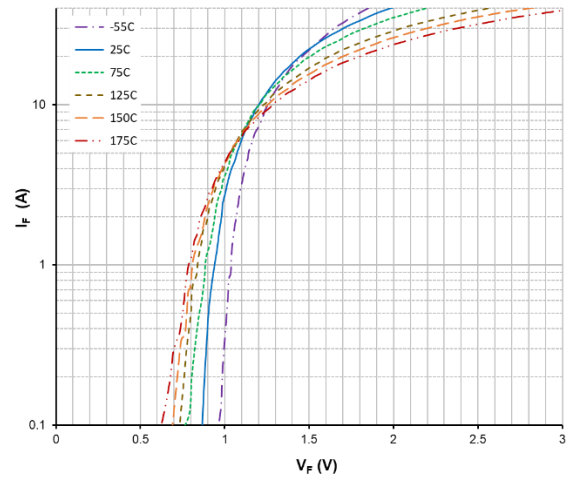
Figure 2. Forward Characteristics
