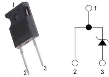
TO-247-2
