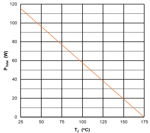
Figure 4. Power Derating
