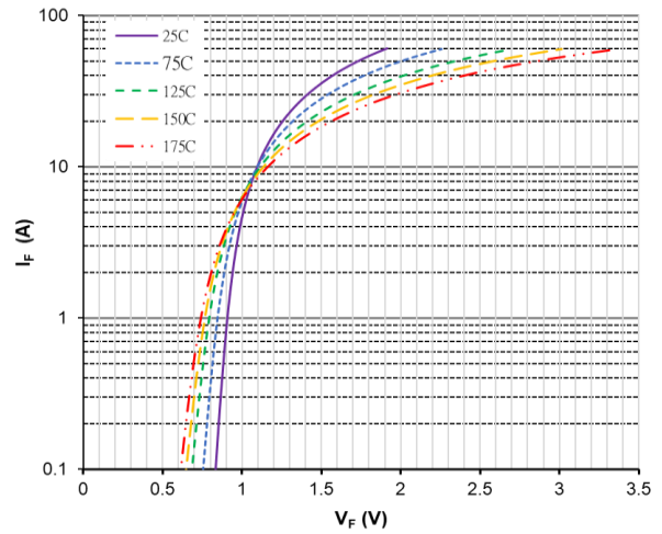
Figure 2. Forward Characteristics
