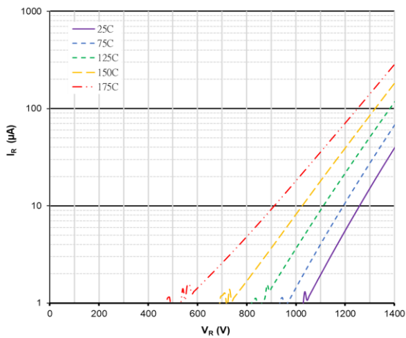
Figure 3. Reverse Characteristics
