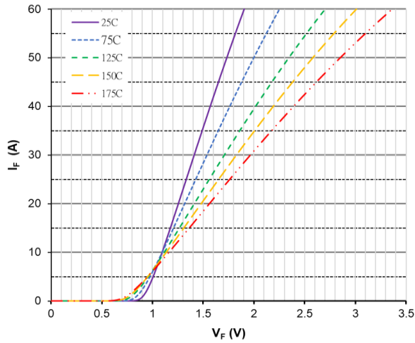
Figure 1. Forward Characteristics
