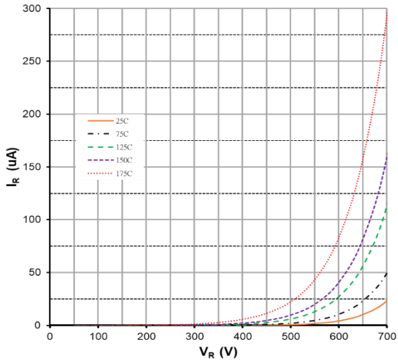
Figure 3. Reverse Characteristics
